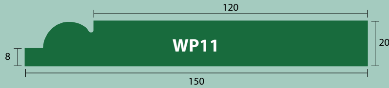
Torus Skirting
