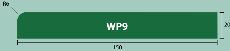
Pencil Round Skirting
