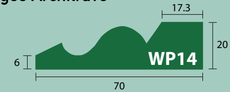
Ogee Architrave
