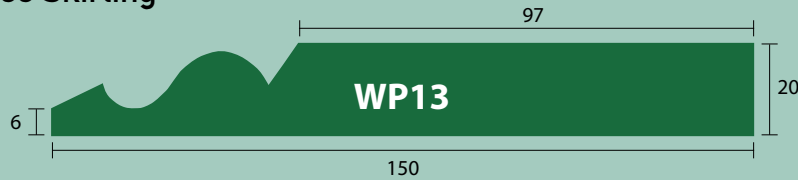
Ogee Skirting
