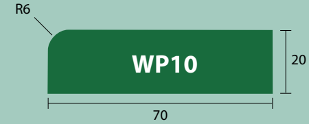
Pencil Round Architrave
